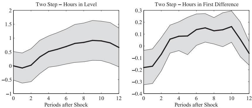
FIG. 6. IRFs of Hours with Business Sector Data.
