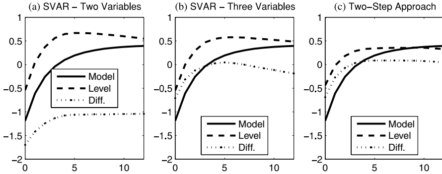
FIG. 1. True and Estimated IRFs of Hours.
