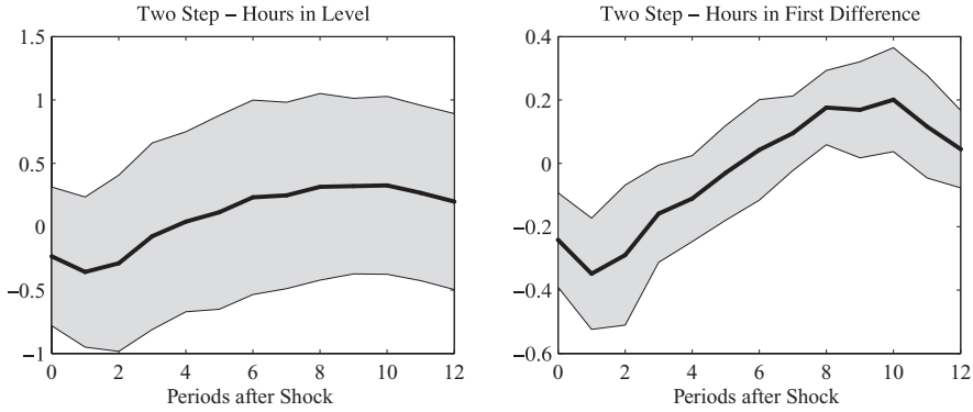
Panel (b). NFB Sector Data and Sample Period 1959Q1–2003Q4
