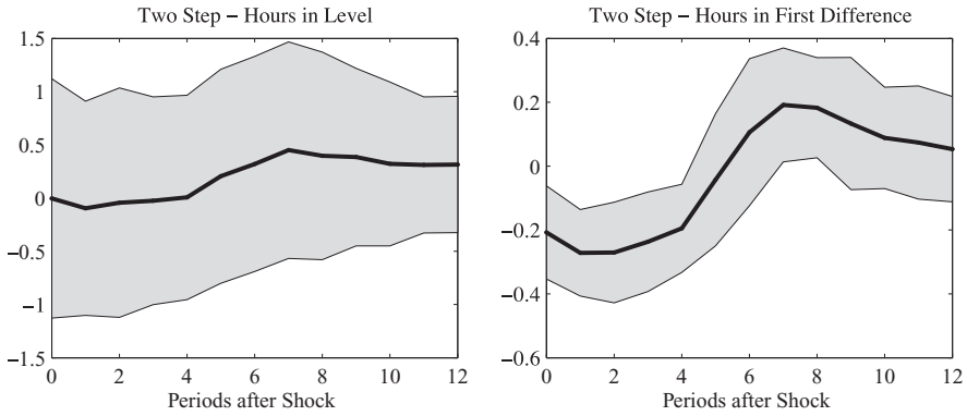
FIG. 10. IRFs of Hours with a Five-Variable System.
