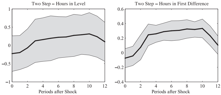
FIG. 8. IRFs of Hours using Investment-to-Output Ratio.
