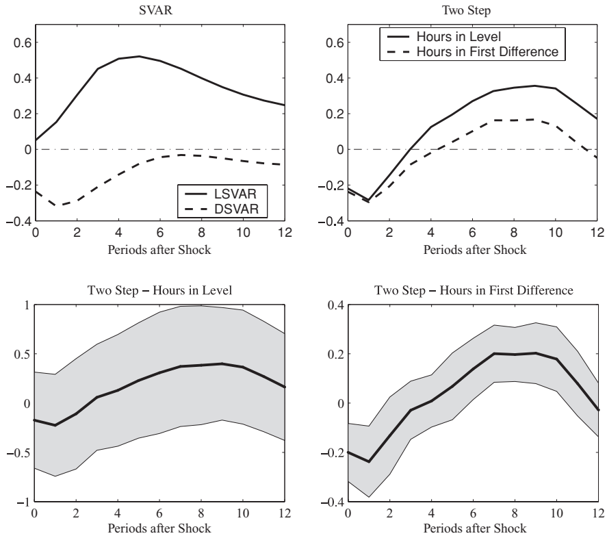
FIG. 4. IRFs of Hours to a Technological Improvement (NBF Data).
