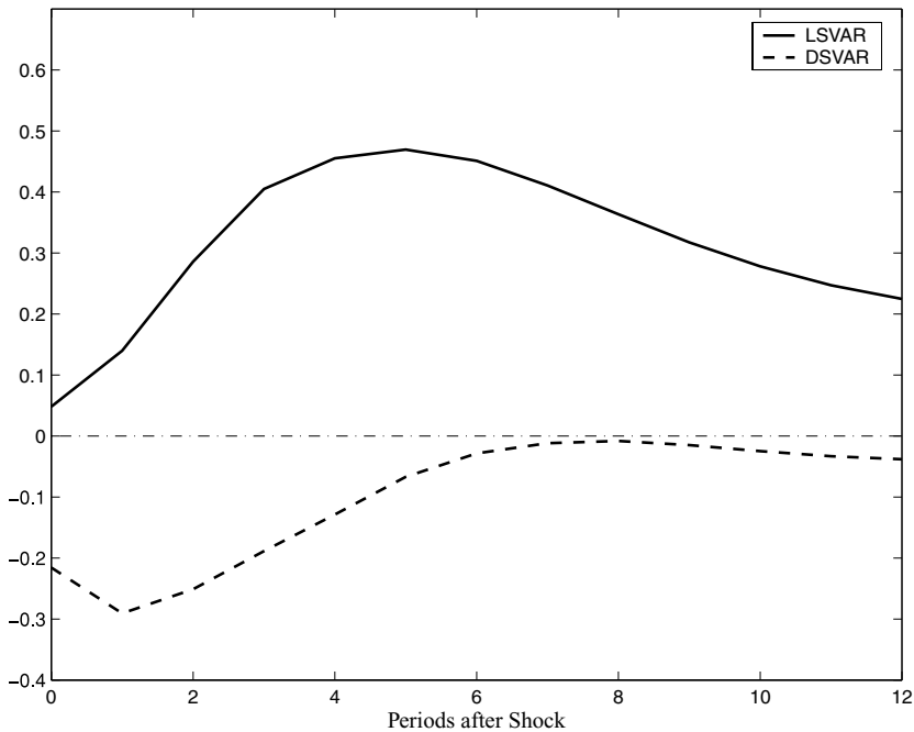
FIG. 5. Three-Variable VARs.
