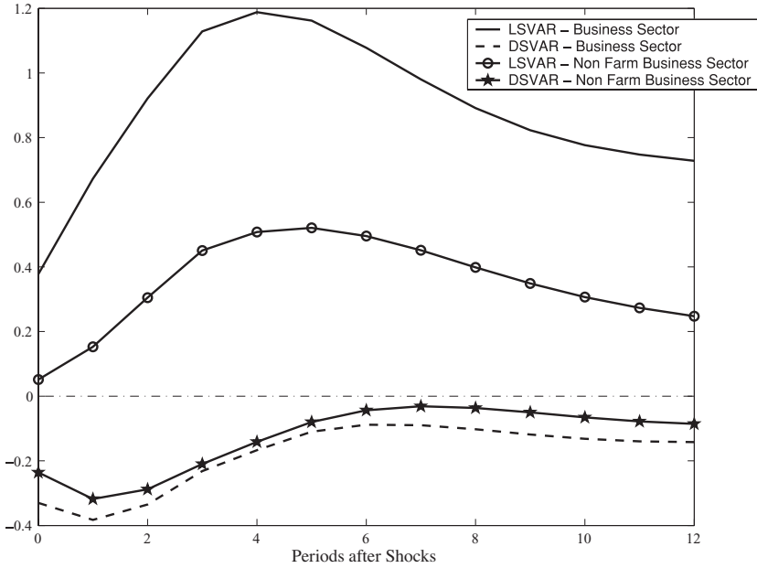
FIG. 7. SVARs with Different Sector Data.
