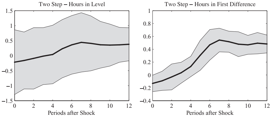
FIG. 11. IRFs of Hours with Breaks in Labor Productivity.
