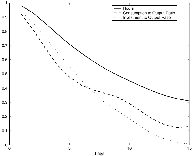
FIG. 3. ACFs.
