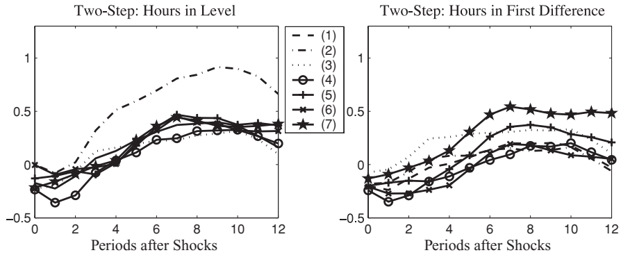
FIG. 12. Summary of the Results; NFB Sector Data and Sample Period Is 1948Q1–2003Q4.
